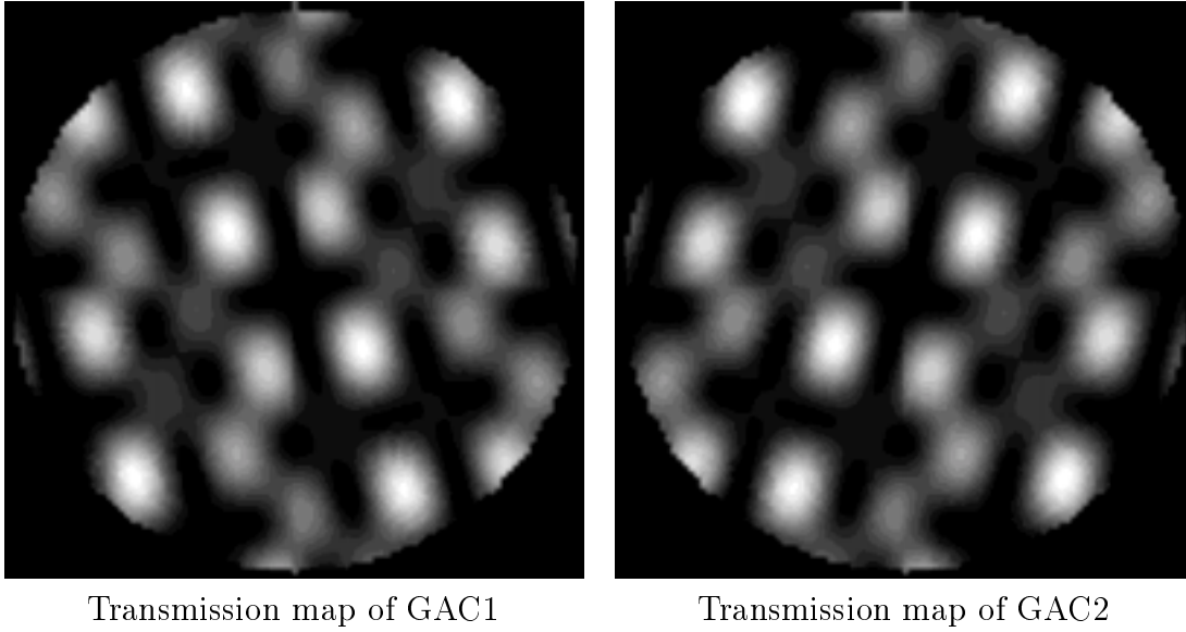
Figure 4.3: RL2(1,0.84,0.54,0,0.70) configuration: transmission maps of the two GACs projected on the sky. Field of view is 500 \times 500 mas, interferometric array radius 15 m, and observing wavelength 10 \mu\text{m} .
