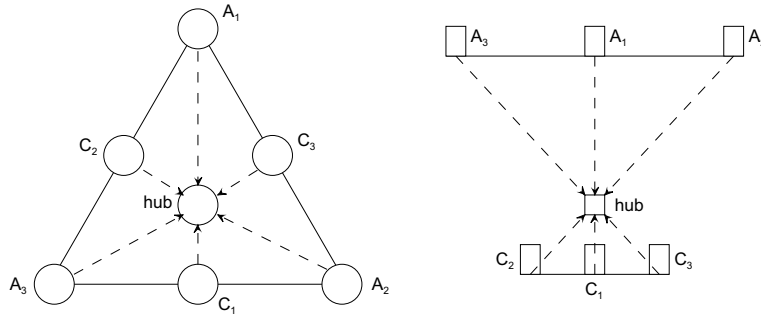
Figure 3.14: 3D Mariotti combination scheme. The six telescopes are lying on a paraboloid, the focus of which is occupied by the central hub.
