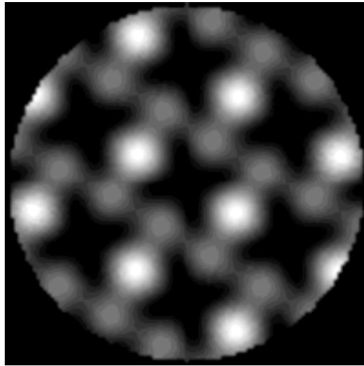
Figure 3.16: Transmission map of GAC1 on the sky. Field of view is 500 \times 500 \text{ mas} , interferometric array radius 15 \text{ m} , and observing wavelength 10 \mu\text{m} .
