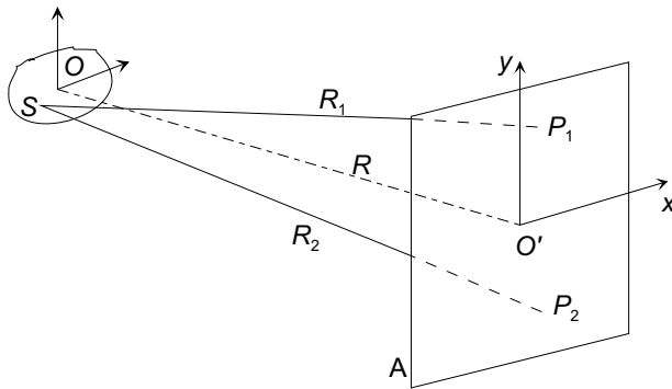
Figure 1.3: Illustrating the van Cittert–Zernicke theorem.
