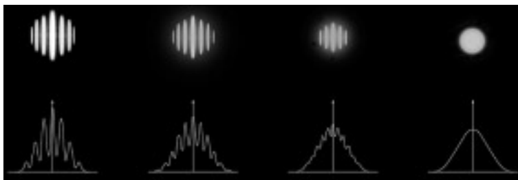
Figure 1.2: Interference fringes for a binary star. From left to right: the contrast between bright and dark fringes progressively decreases as the baseline increases, until the moment where it cancels and the two sources are resolved (ESO PR Photo 10e/01).
