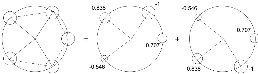
Figure 4.1: The RL2(1,0.84,0.54,0,0.70) nulling interferometer and its two sub-nulling interferometers, the GACs, with their generalized entrance pupils.
