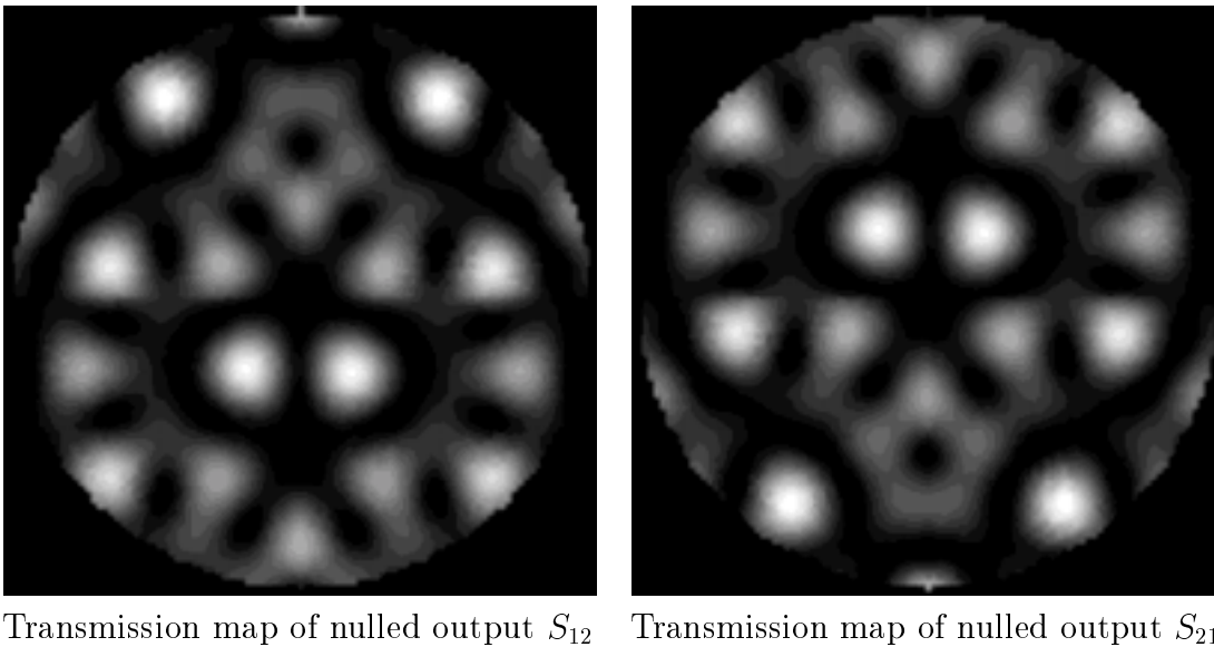
Figure 4.4: RL2(1,0.84,0.54,0,0.70) configuration: transmission maps of nulled output from GAC1 recombined with nulled output from GAC2, with a phase shift of \pi/2 (left) and -\pi/2 (right).
