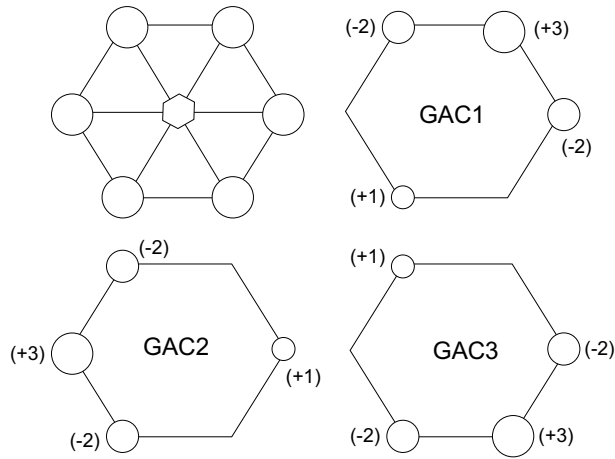
Figure 3.15: The RL3(3,2,0,1,0,2) interferometer and its three sub-nulling arrays with their generalized entrance pupils.
