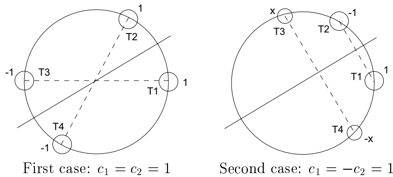
Figure 4.8: Generalized entrance pupil for the two cases considered above ( T_k is the telescope's number in GAC1). Only the second case can give rise to a RL interferometer, when combined with one of its two “complementary” GACs.
