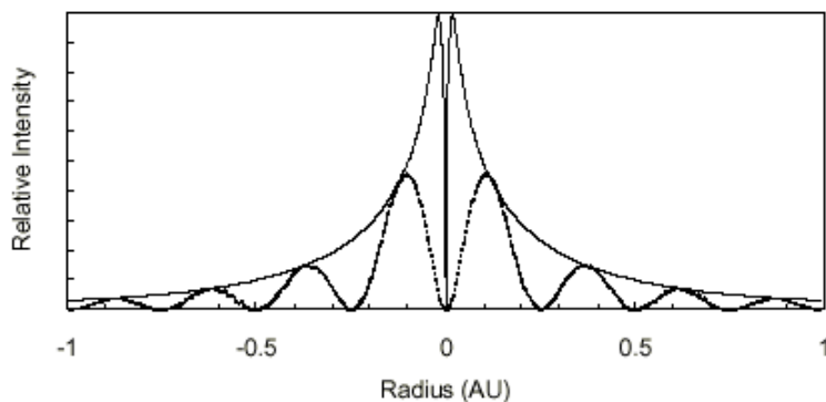
Figure 3.5: Cross-sectional view through an edge-on exo-zodiacal cloud at distance 10 pc, showing the emergent flux and the flux transmitted by the 10\ \mu\text{m} fringe pattern of the Keck interferometer in the nulling mode (from [28]).
