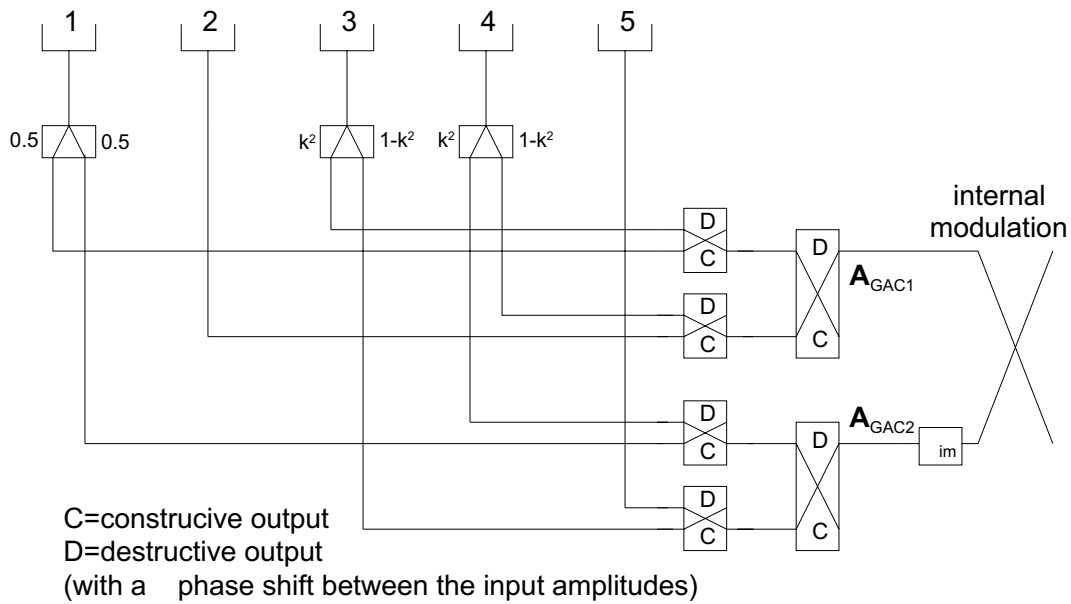
Figure 4.2: Schematic recombination of the beams for the RL2(1,0.84,0.54,0,0.70) interferometer. Note the beam-splitter intensity coefficients of k^2 , 1 - k^2 (where k = 0.838 ).
