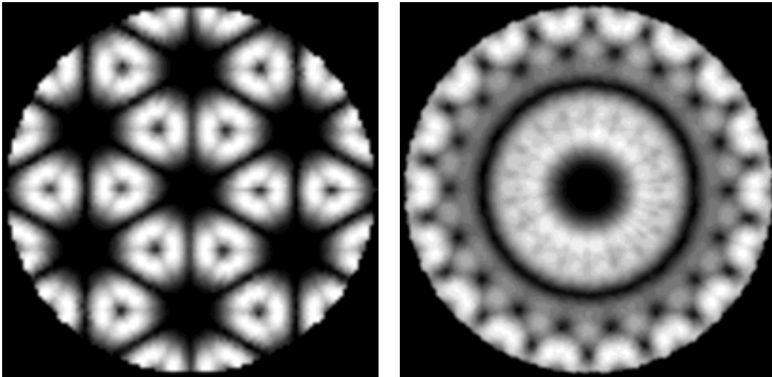
Figure 3.18: Left: modulation efficiency map. Right: mean modulation efficiency when superimposing three maps obtained by 20^\circ successive rotations. Note that azimuthal directions of zero modulation are not present any more.
