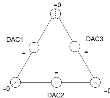
Figure 3.13: Geometry of the Mariotti nulling interferometer. Dotted lines indicates telescopes which are shared between adjacent sub-arrays. Note that the area ratio is 1:2:1 for each DAC, so that the diameter ratio is 1:\sqrt{2}:1 , in agreement with the remark on DAC's recombination (section 3.2.2). The recombination scheme of figure 3.8 is used for each individual DAC with equal size telescopes and 50:50 beam-splitters behind each summit telescope.
