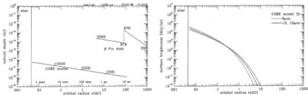
Figure 5.1: Thermal model of a 1-zodi cloud around a Solar-type star viewed from 10 pc based on the COBE zodiacal model (from Backman [4]). Left: Disk vertical optical depth and temperature versus distance from the central star, compared with a possible profile of the cold dust disk of \beta Pic. Right: Thermal emission surface brightness for several wavelengths around 10 \mu\text{m} .
