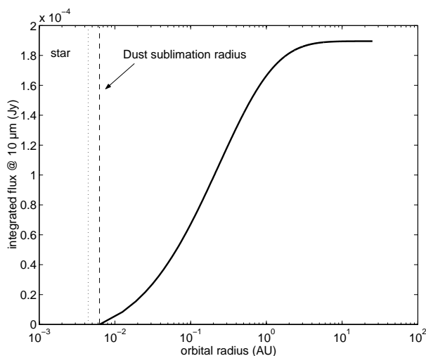
Figure 5.2: Integrated flux at 10 \mu\text{m} versus distance from the star for a 1-zodi cloud around a Solar-type star viewed from 10 pc, based on the IRAS zodiacal model. Note that 90% of the flux comes from the region between 0.01 and 1 AU.
