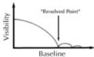
Figure 1.8: Fringe visibility vs. baseline. Measurements of low visibilities are necessary in order to characterize the source, but unfortunately these measurements are the less accurate.
