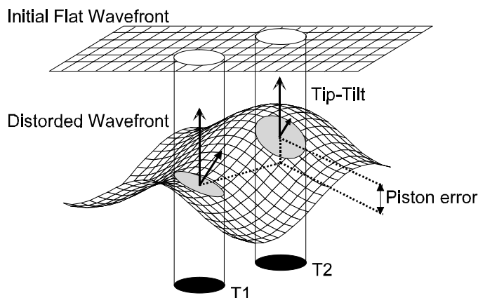
Figure 1.9: Wavefront distortion induced by atmospheric turbulence (from Paresce [45]).
