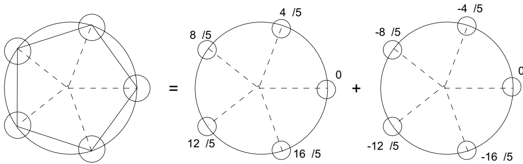
Figure 4.30: The Nils interferometer with its two sub-nulling arrays. The applied phase shifts are indicated near each telescope for each sub-interferometer.
