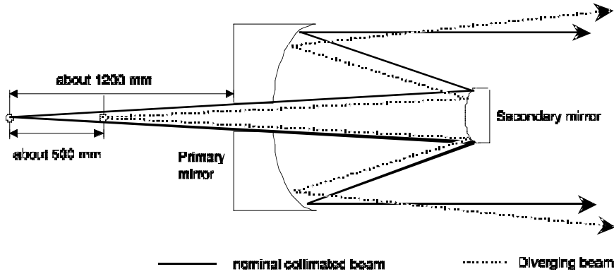
FIGURE 8 : DE-FOCUSING PRINCIPLE
